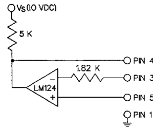
Figure 2 Sensing Bridge Supply Circuit
